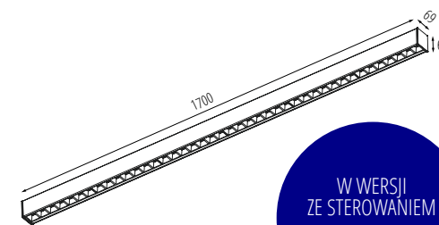
ALD-RST-L-NT: 1700mm
