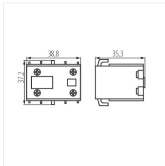
KCPM-AX11
