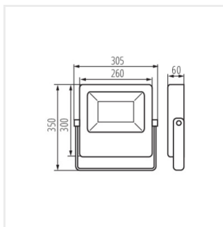
FL AGOR/A LED 150W NW
