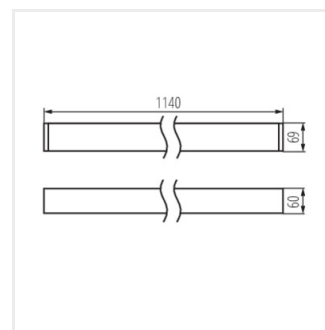
ALD-MH5D-WW-RST-W-NT
