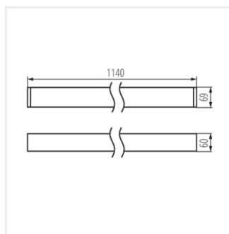
ALD-MH5D-NW-RST-W-NT
