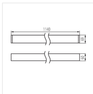
ALD-MH5D-NW-RST-B-NT
