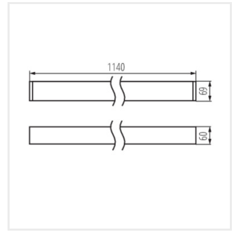
ALD-MS-NW-RST-W-NT
