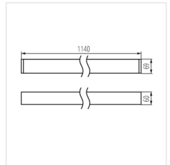
ALD-MS5D-WW-RST-W-NT
