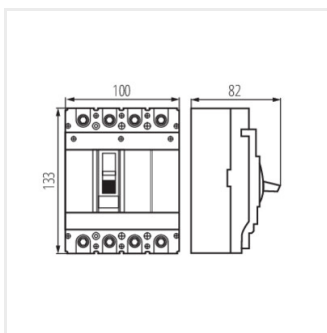
KMCCB-RT-125A-4P
