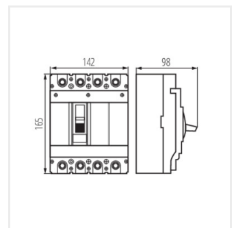
KMCCB-RT-250A-4P
