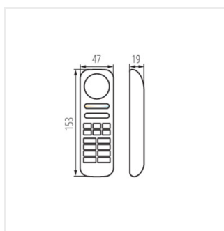
REMOTE 8 RGB/CCT-W
