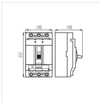
KMCCB-RT-400A
