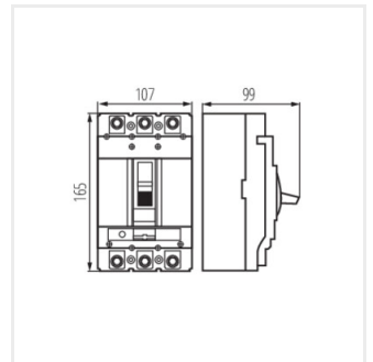
KMCCB-RT-250A
