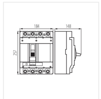
KMCCB-RT-400A-4P-H
