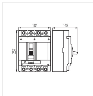
KMCCB-RT-400A-4P
