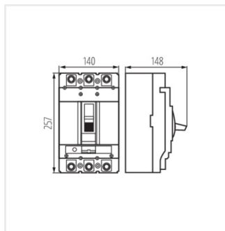
KMCCB-RT-400A-H
