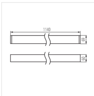
ALD-MH5D-NW-RST-B-NT
