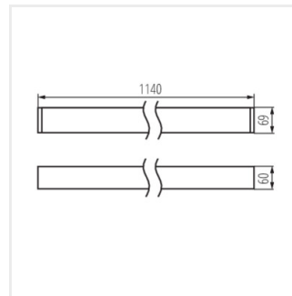
ALD-MH-WW-RST-B-NT
