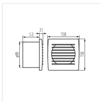
AERO RK100
