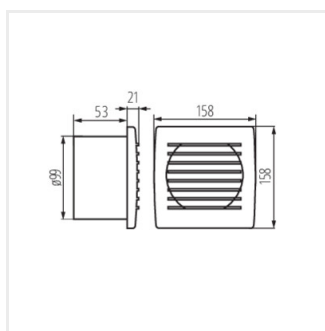
AERO RK100T
